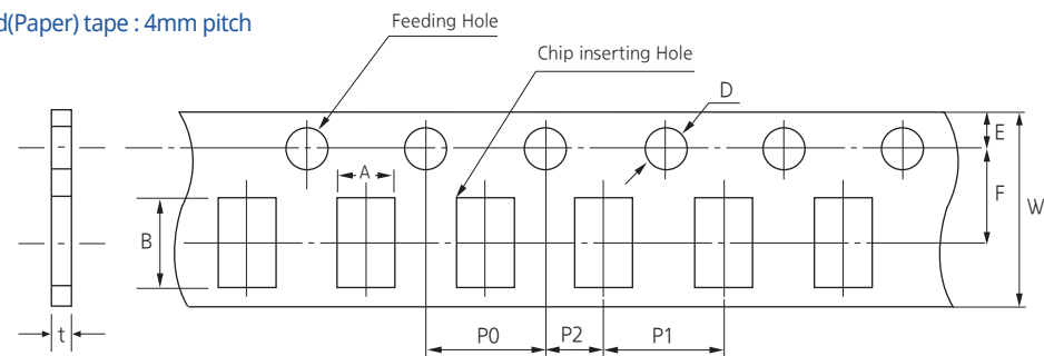
Cardboard(Paper) tape : 4mm pitch
