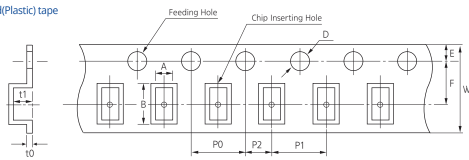
Embossed(Plastic) tape
